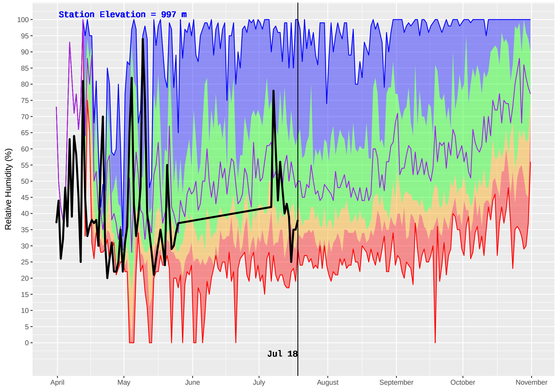
JERRY (190) : Historical (1988–2016) and Current (2018) Daily Relative Humidity
