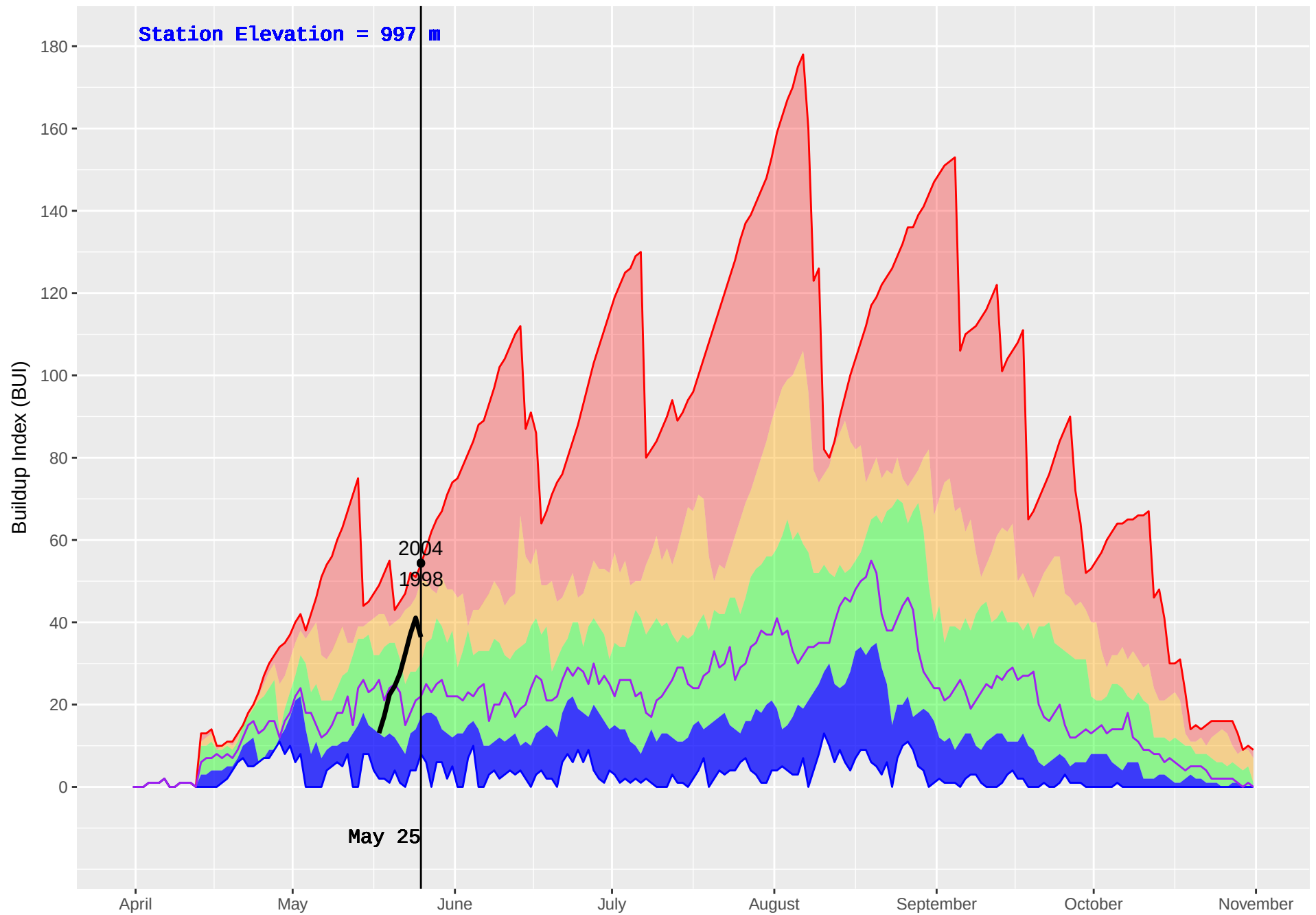
JERRY (190) : Historical (1988–2016) and Current (2018) Daily Buildup Index (BUI)
